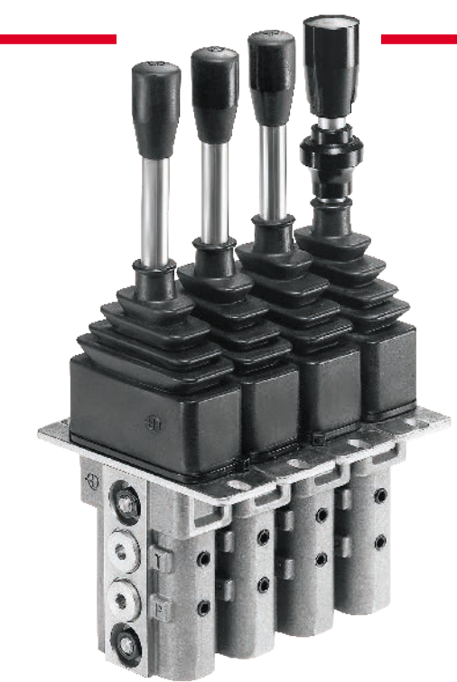
液壓引導式手柄 Joystick
